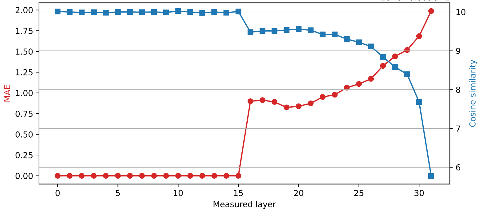
SmolLM2-360M | Quantized layer 15 | float32 → int2 1e-5+9.999e-1
