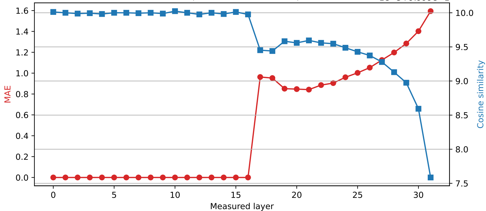
SmolLM2-360M | Quantized layer 16 | float32 \rightarrow int2 1e-5+9.999e-1
