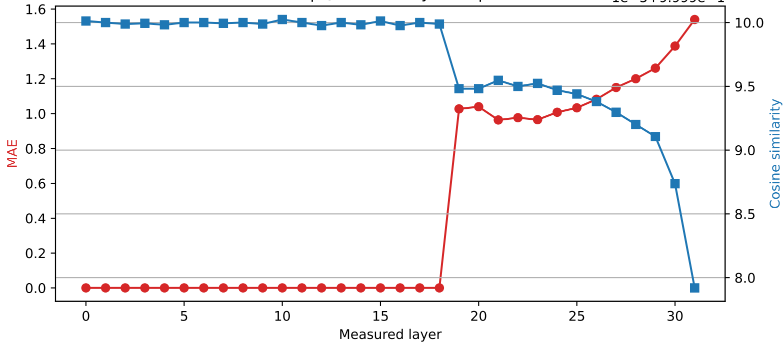
SmolLM2-360M | Quantized layer 18 | float32 \rightarrow int2 1e-5+9.999e-1
