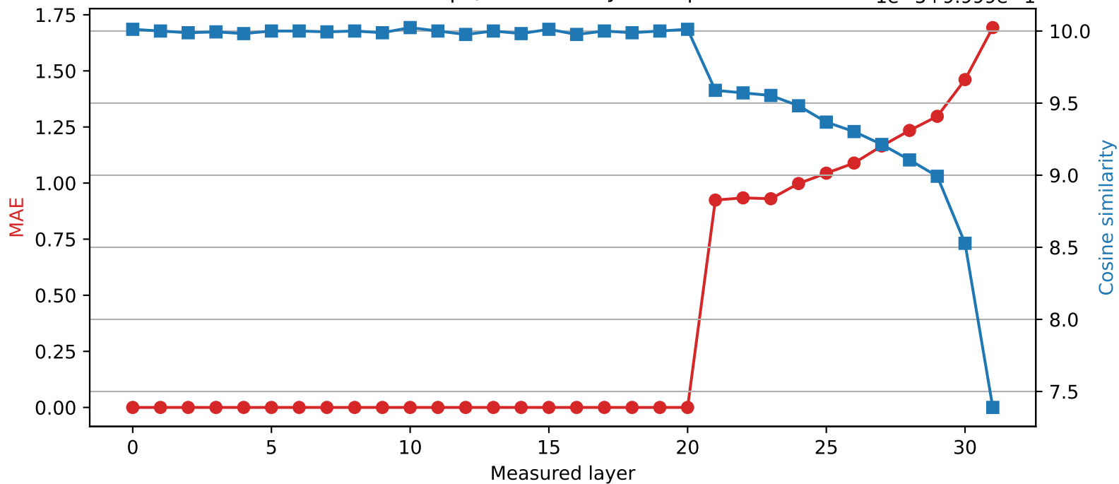
SmolLM2-360M | Quantized layer 20 | float32 → int2 1e-5+9.999e-1
