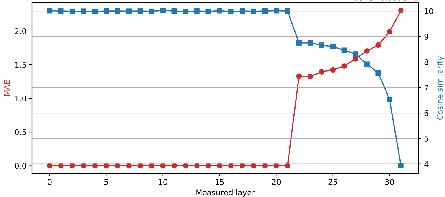
SmolLM2-360M | Quantized layer 21 | float32 \rightarrow int2 1e-5+9.999e-1
