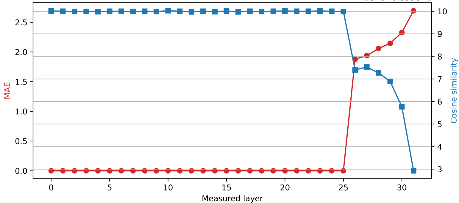
SmolLM2-360M | Quantized layer 25 | float32 \rightarrow int2 1e-5+9.999e-1
