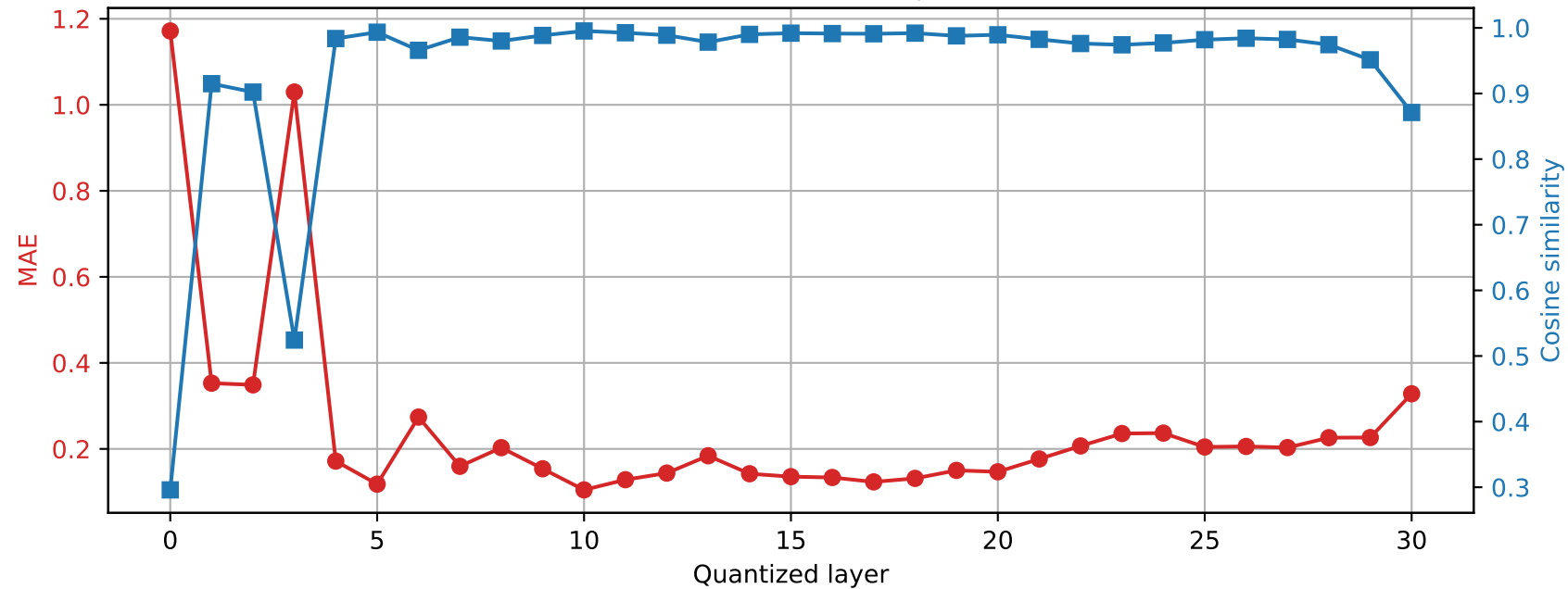
SmolLM2-360M | Prompt 1 Final RMSNorm output damage | float32 → int2
