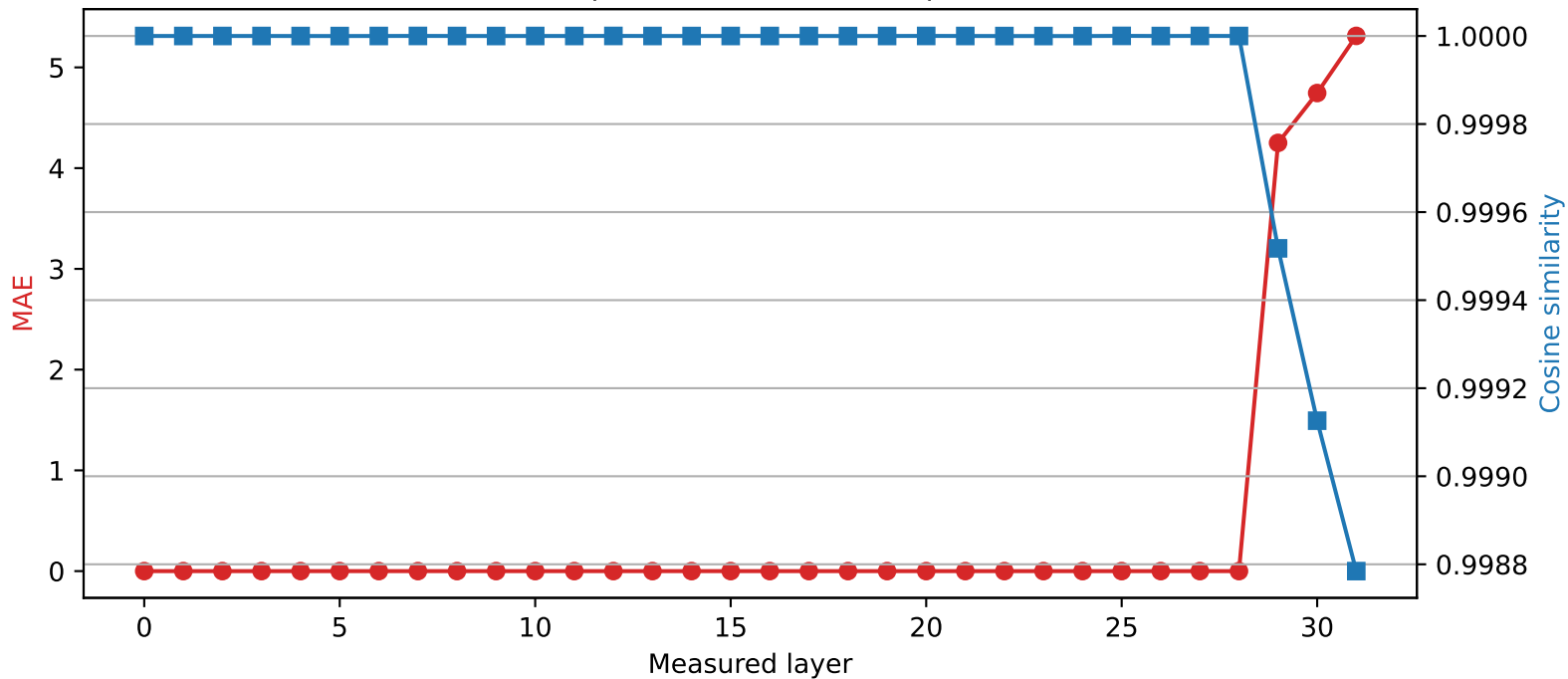
SmolLM2-360M | Quantized layer 28 | float32 → int2
