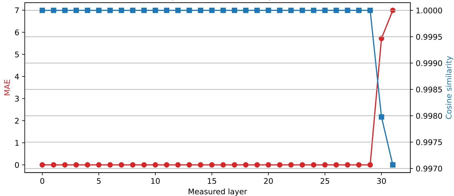
SmolLM2-360M | Quantized layer 29 | float32 \rightarrow int2
