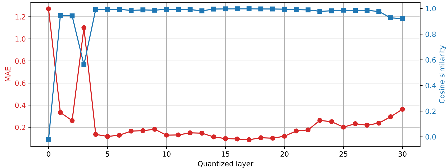
SmolLM2-360M | Prompt 2 Final RMSNorm output damage | float32 \rightarrow int2
