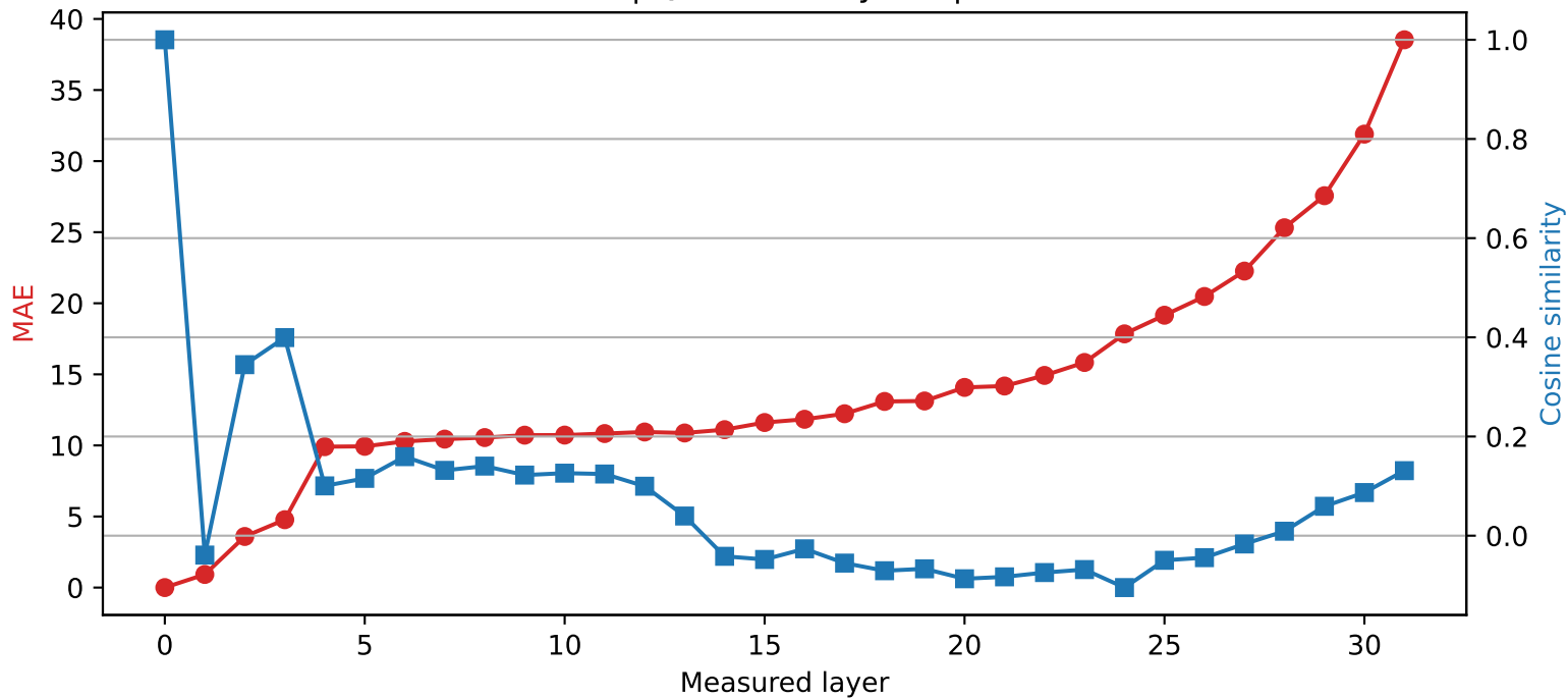
SmolLM2-360M | Quantized layer 0 | float32 → int2
