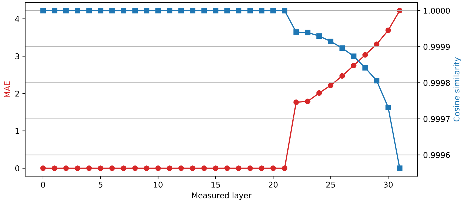
SmolLM2-360M | Quantized layer 21 | float32 → int2
