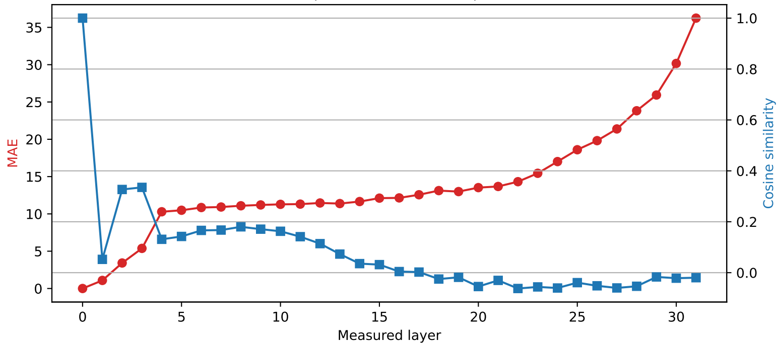
SmolLM2-360M | Quantized layer 0 | float32 \rightarrow int2
