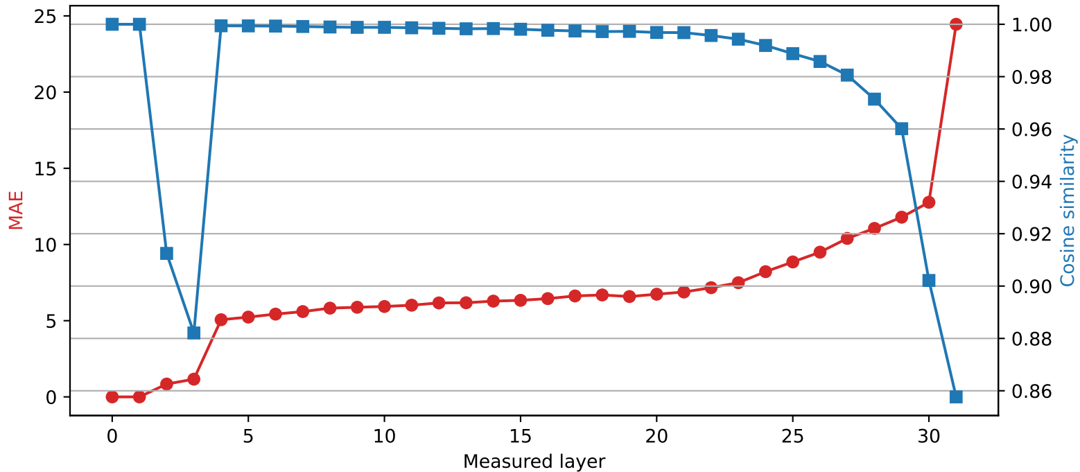
SmolLM2-360M | Quantized layer 1 | float32 → int2
