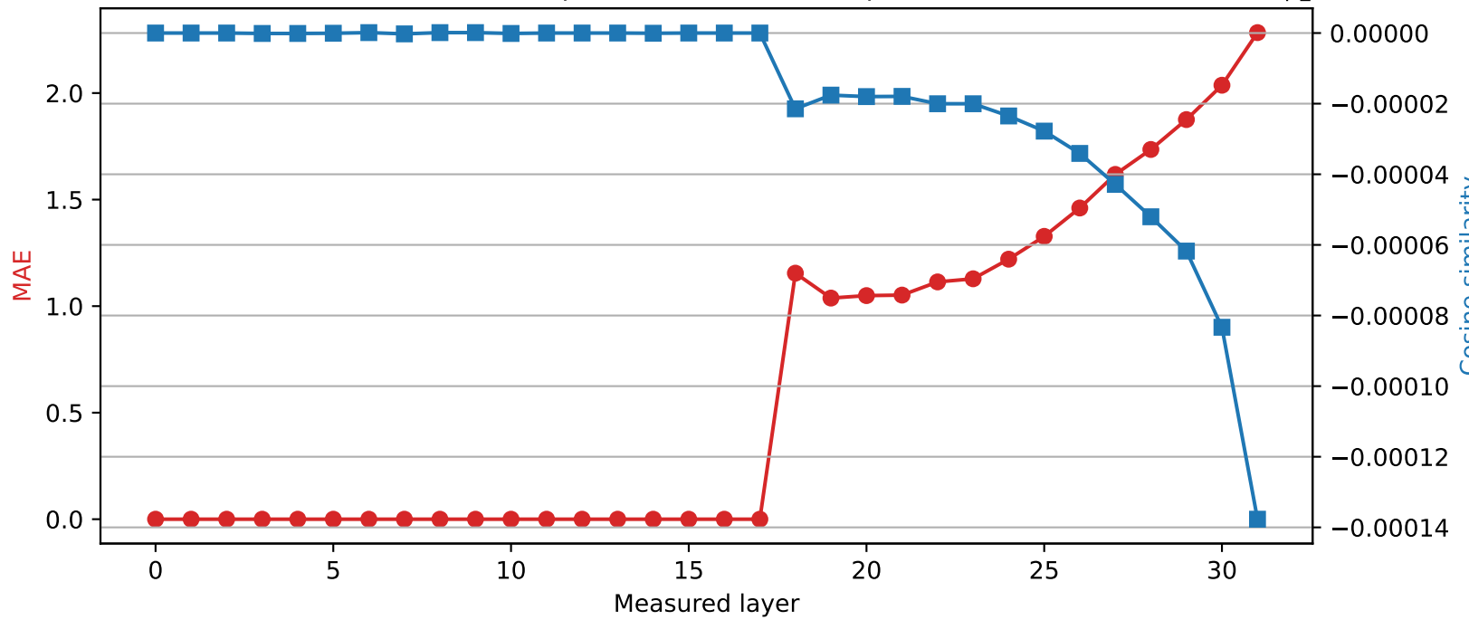
SmolLM2-360M | Quantized layer 17 | float32 \rightarrow int2
