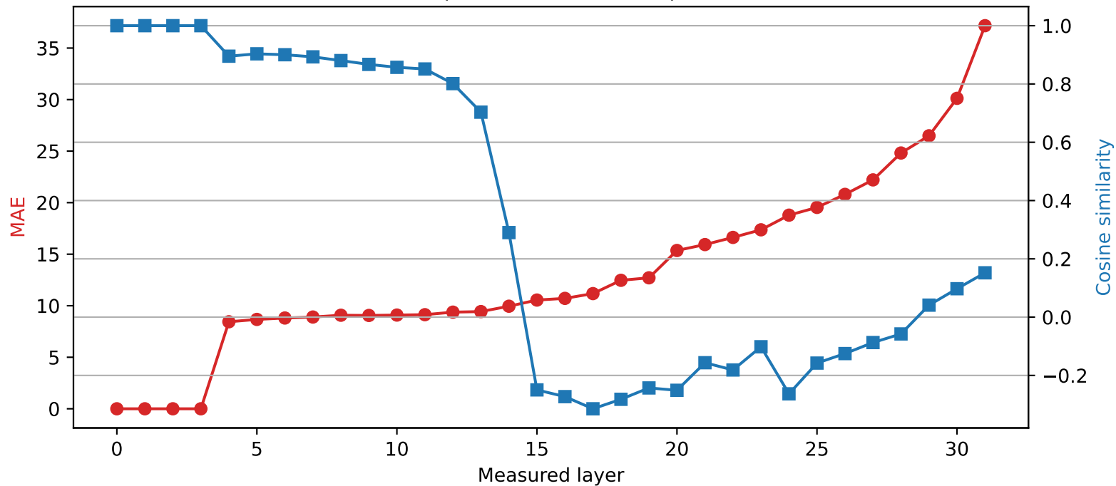
SmolLM2-360M | Quantized layer 3 | float32 \rightarrow int2
