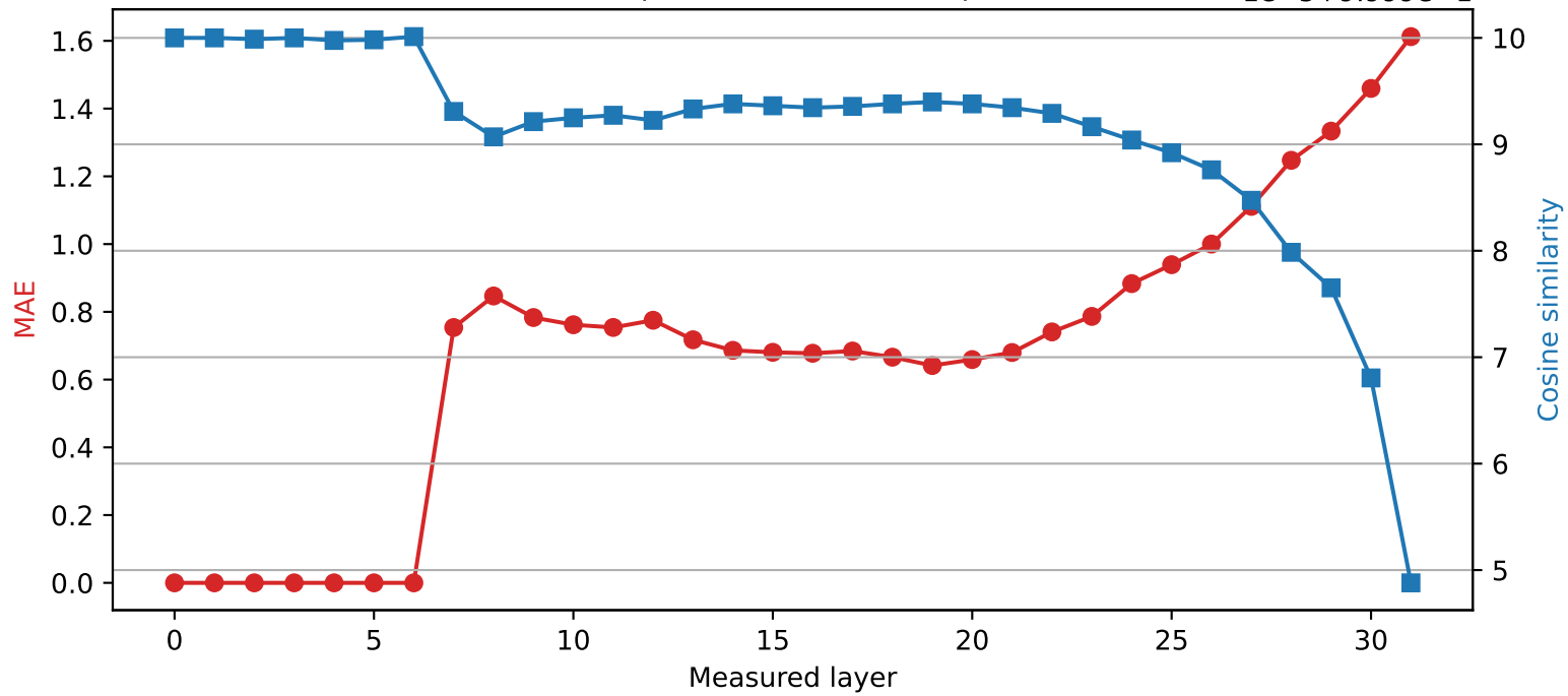
SmolLM2-360M | Quantized layer 6 | float32 \rightarrow int2
