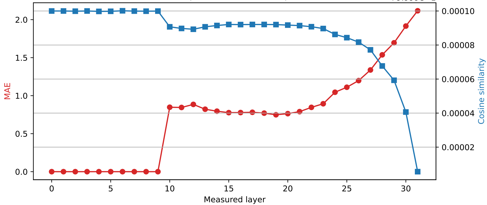
SmolLM2-360M | Quantized layer 9 | float32 \rightarrow int2
