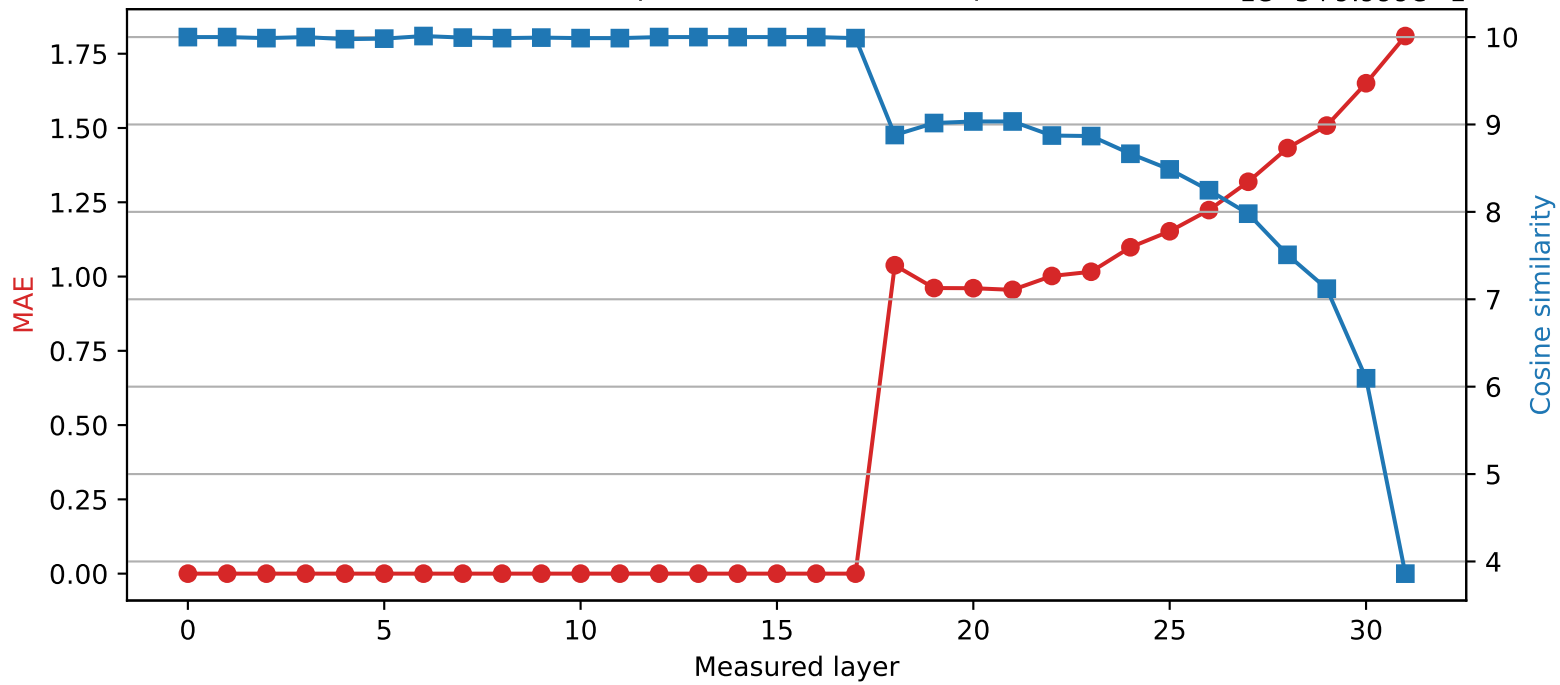
SmolLM2-360M | Quantized layer 17 | float32 \rightarrow int2 1e-5+9.999e-1
