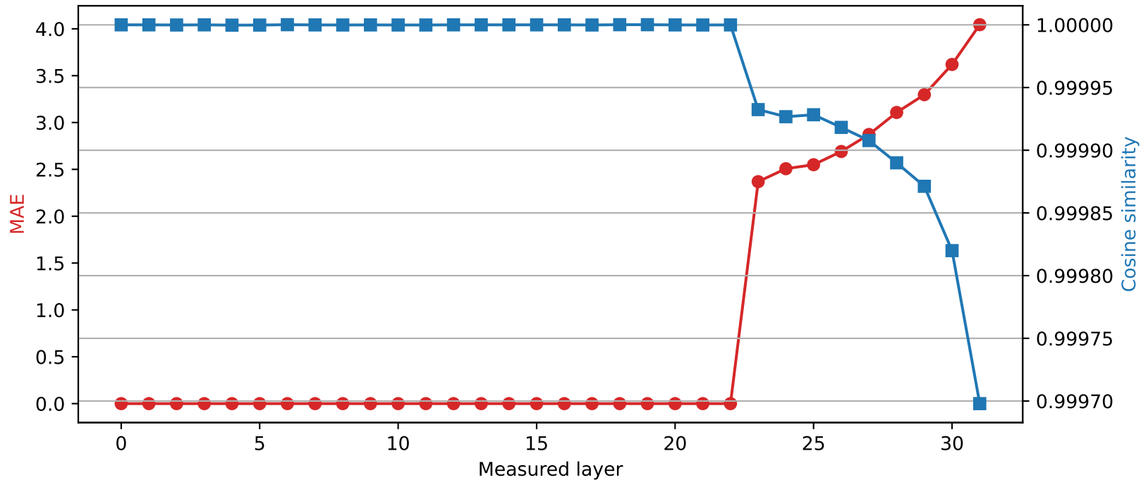
SmolLM2-360M | Quantized layer 22 | float32 → int2
