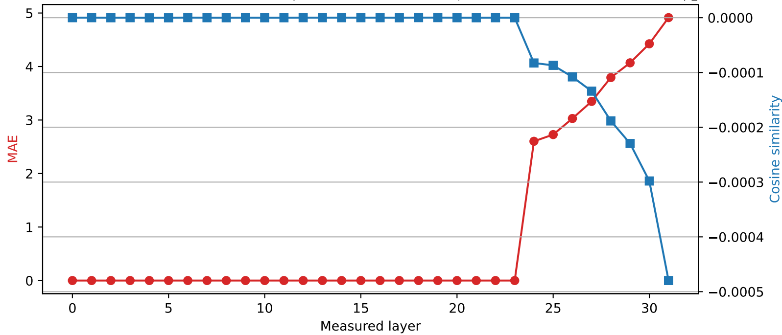
SmolLM2-360M | Quantized layer 23 | float32 \rightarrow int2
