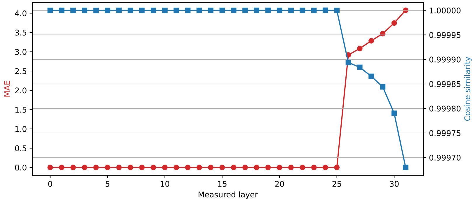
SmolLM2-360M | Quantized layer 25 | float32 \rightarrow int2
