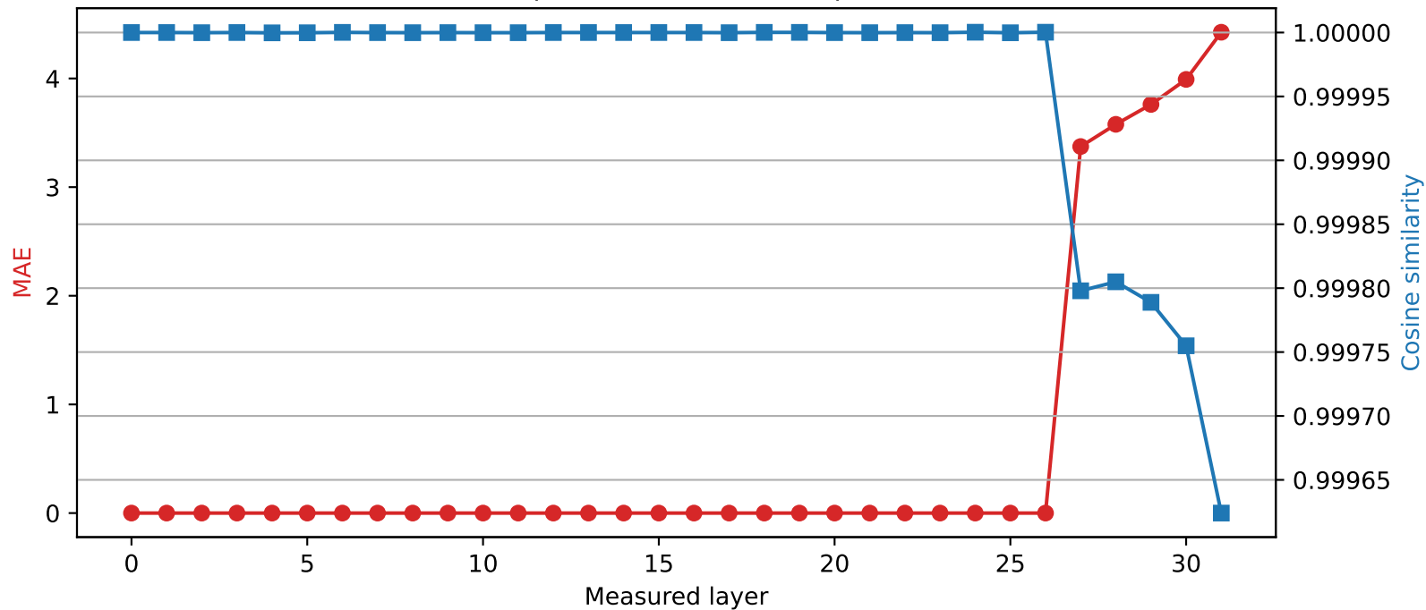
SmolLM2-360M | Quantized layer 26 | float32 → int2
