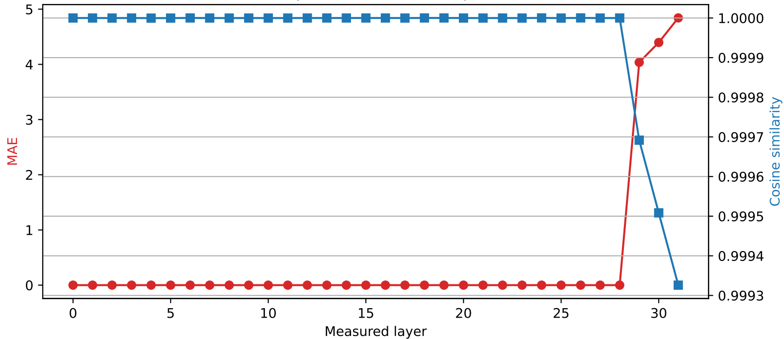
SmolLM2-360M | Quantized layer 28 | float32 \rightarrow int2
