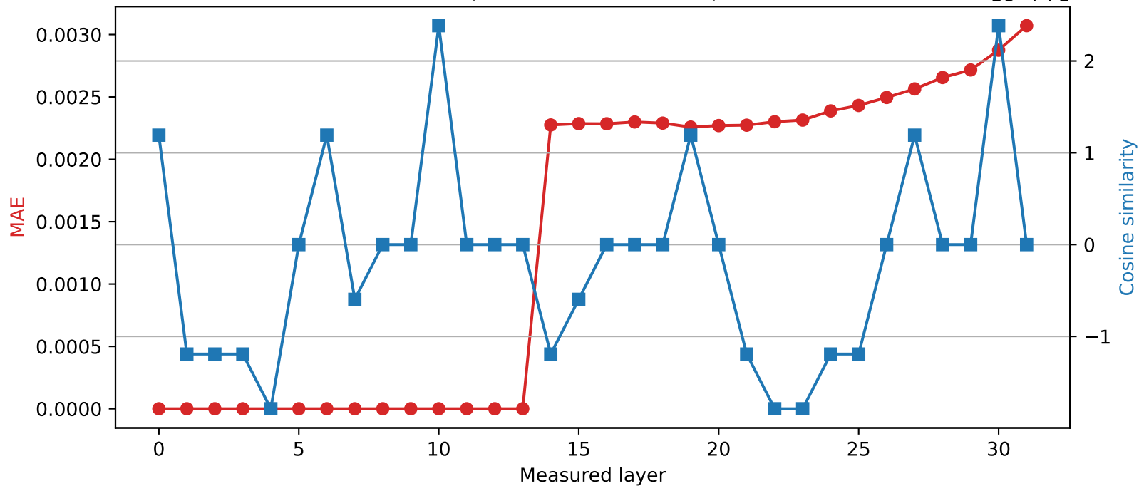
SmolLM2-360M | Quantized layer 13 | float64 \rightarrow int16
