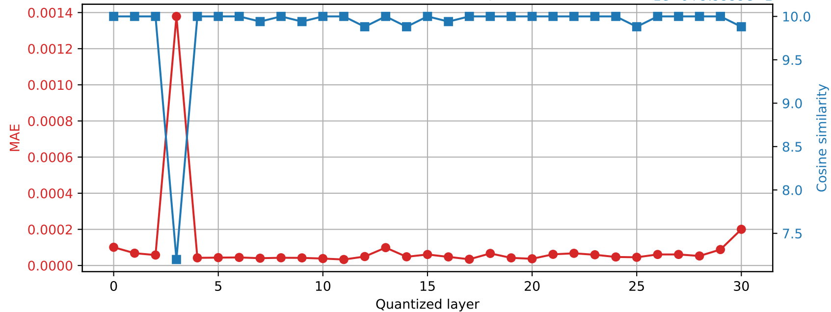
SmolLM2-360M | Prompt 1 Final RMSNorm output damage | float64 → int16
