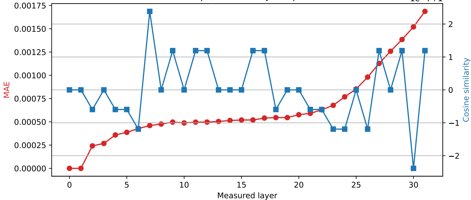
SmolLM2-360M | Quantized layer 1 | float64 → int16
