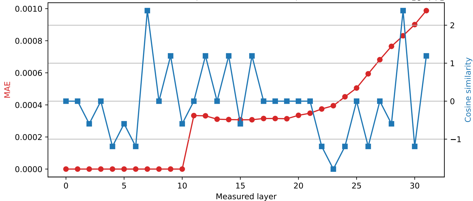
SmolLM2-360M | Quantized layer 10 | float64 \rightarrow int16
