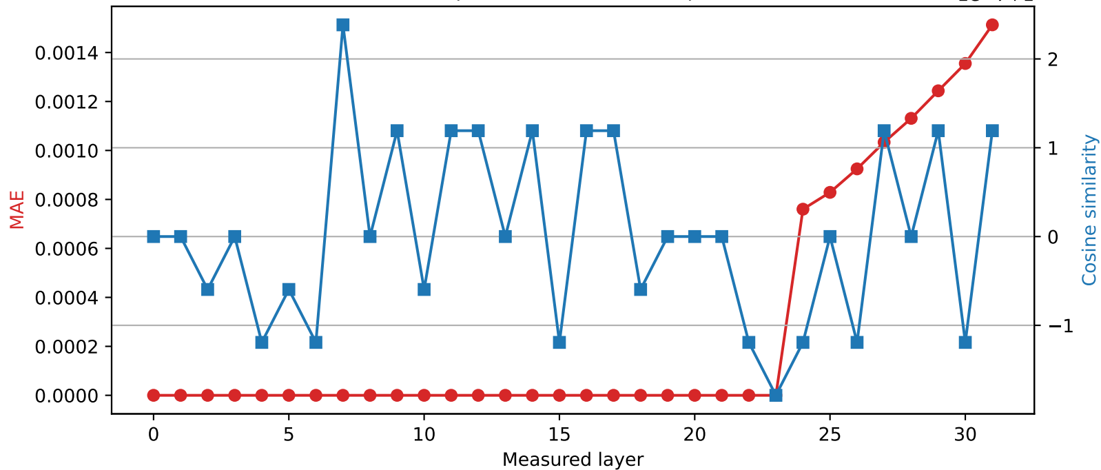
SmolLM2-360M | Quantized layer 23 | float64 \rightarrow int16
