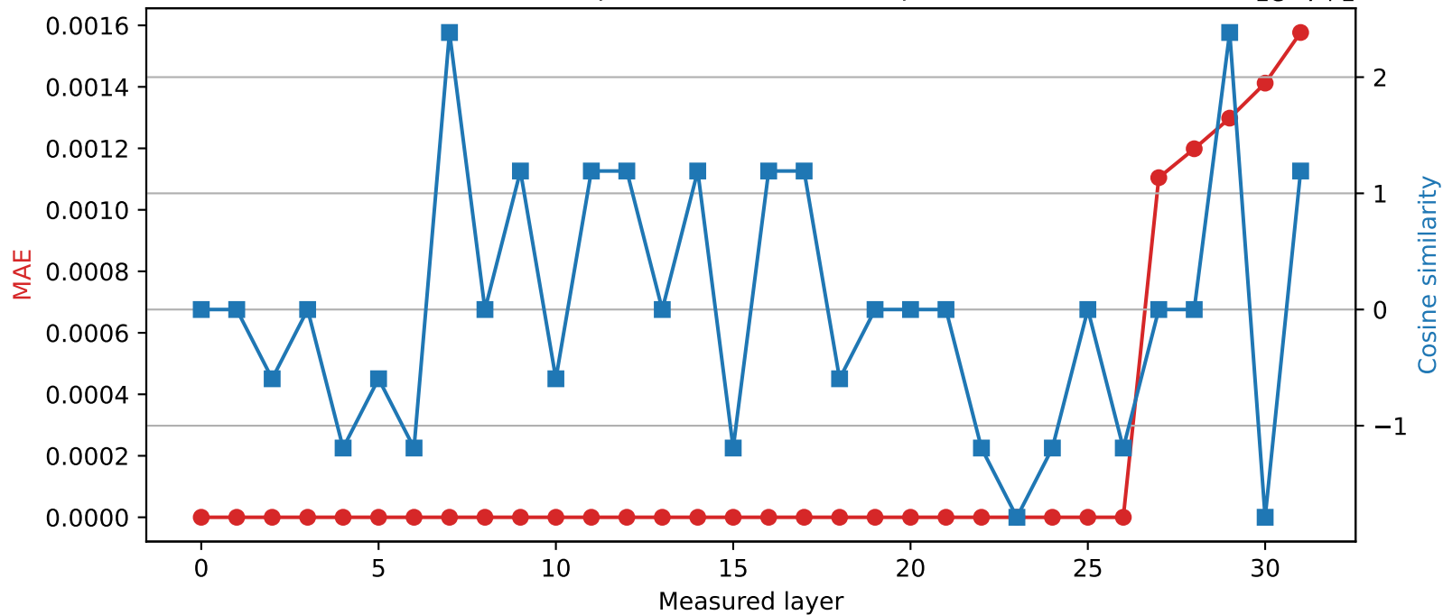
SmolLM2-360M | Quantized layer 26 | float64 \rightarrow int16
