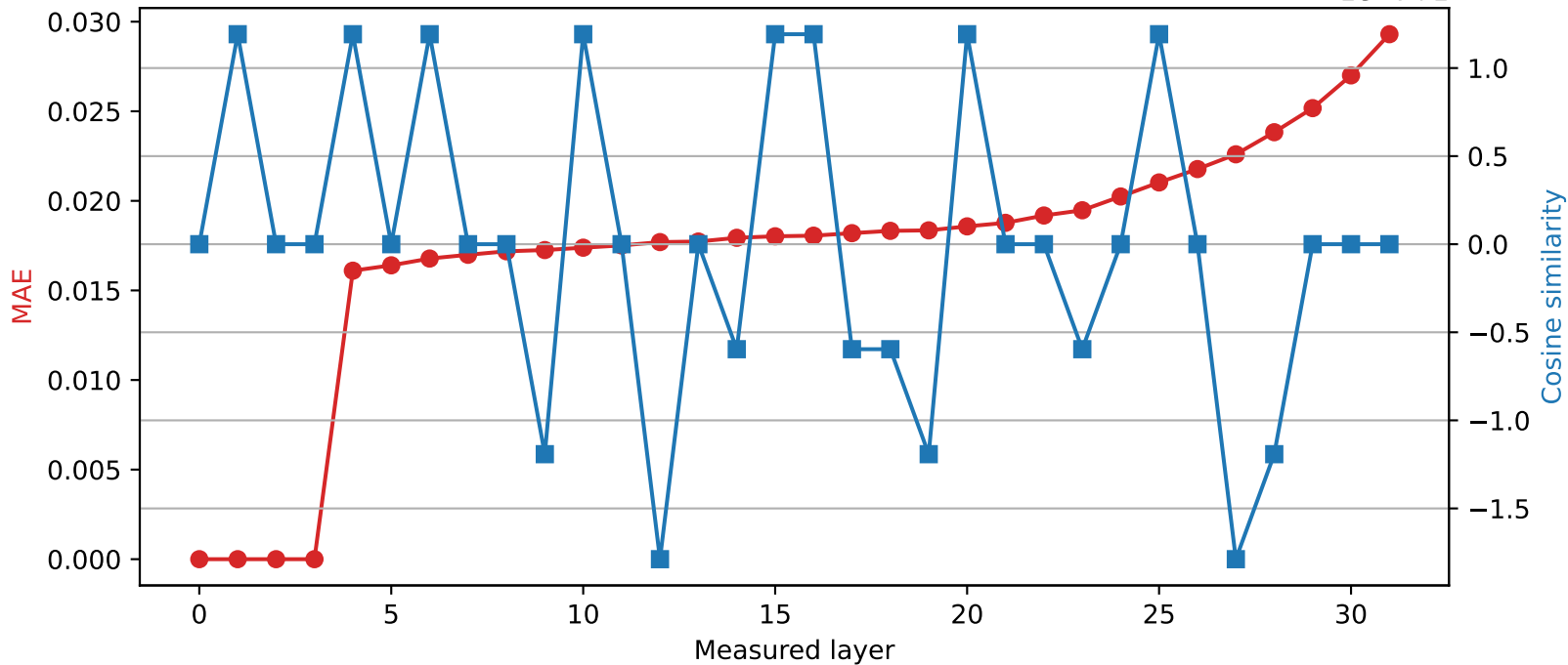
SmolLM2-360M | Quantized layer 3 | float64 → int16
