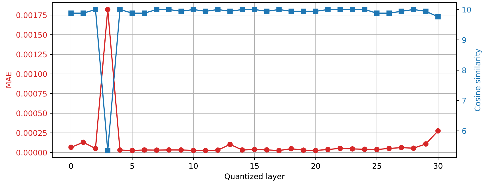
SmolLM2-360M | Prompt 3 Final RMSNorm output damage | float64 → int16
