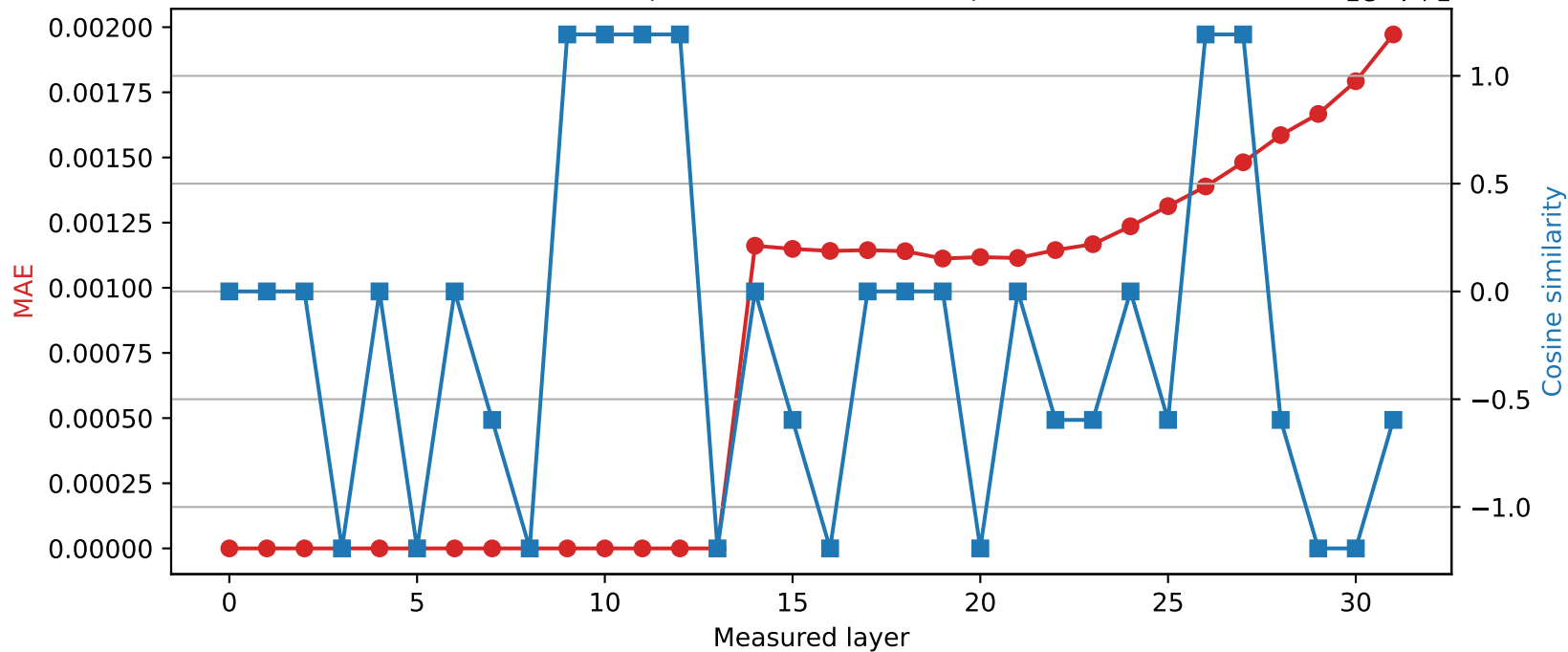
SmolLM2-360M | Quantized layer 13 | float64 → int16
