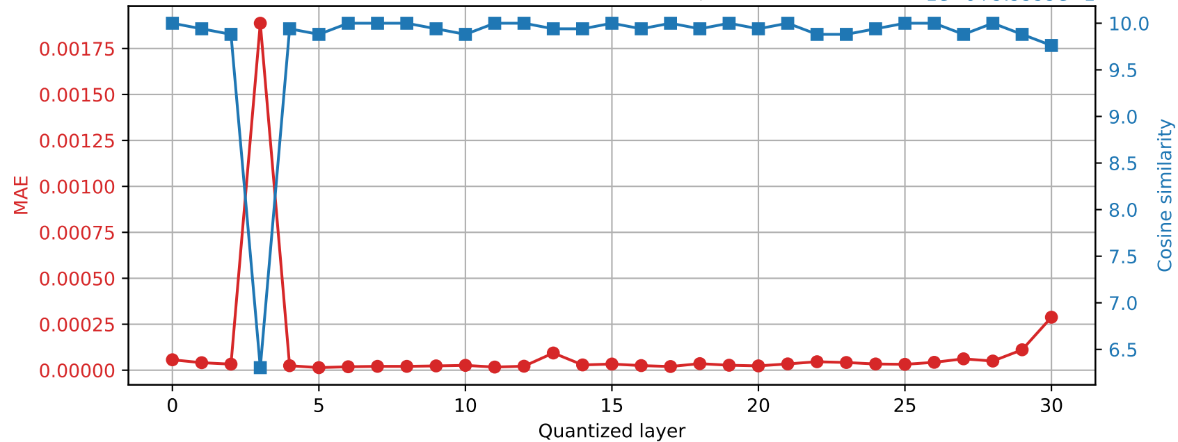
SmolLM2-360M | Prompt 4 Final RMSNorm output damage | float64 → int16
