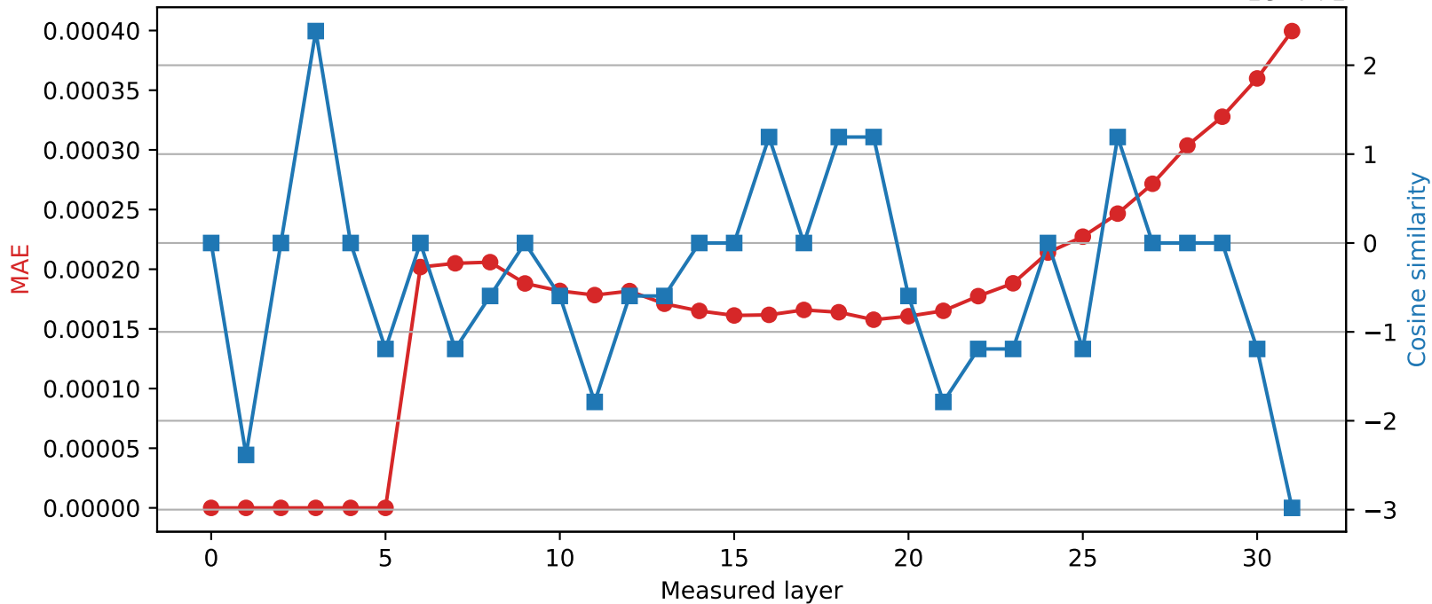
SmolLM2-360M | Quantized layer 5 | float64 → int16
