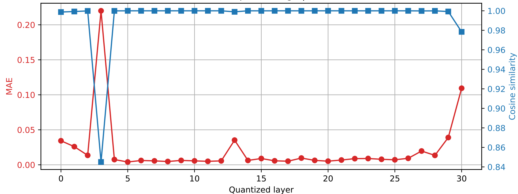
SmolLM2-360M | Prompt 0 Final RMSNorm output damage | float64 → int8
