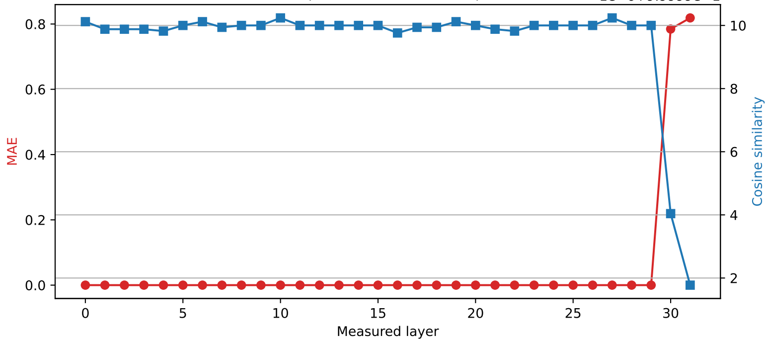
SmolLM2-360M | Quantized layer 29 | float64 → int8 1e-6 + 9.9999e-1
