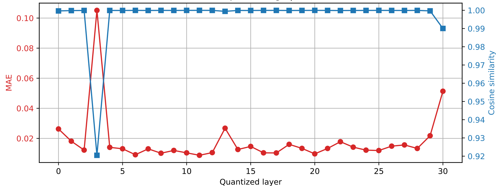
SmolLM2-360M | Prompt 1 Final RMSNorm output damage | float64 → int8
