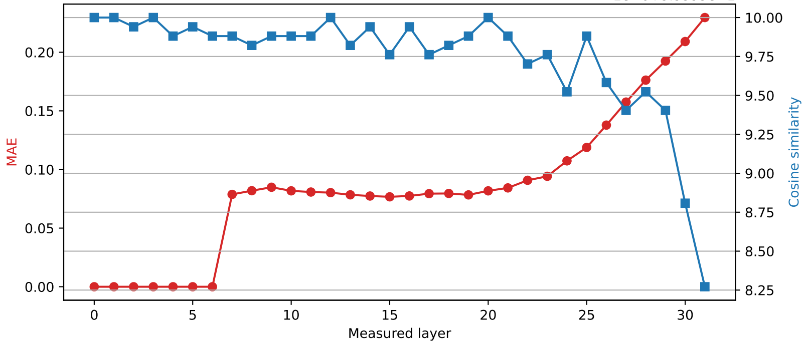
SmolLM2-360M | Quantized layer 6 | float64 → int8 1e-6 + 9.9999e-1
