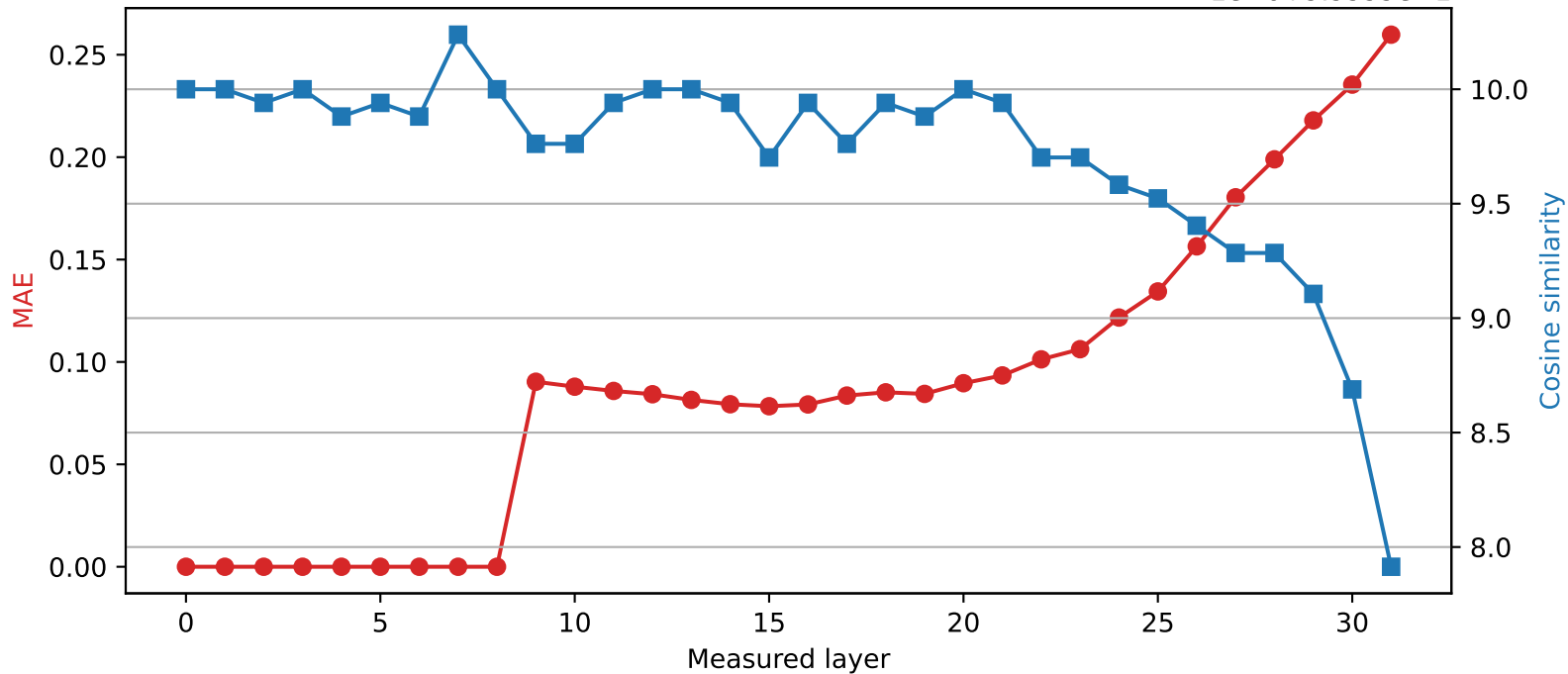
SmolLM2-360M | Quantized layer 8 | float64 → int8 1e-6+9.9999e-1
