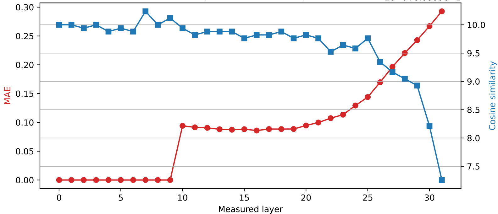
SmolLM2-360M | Quantized layer 9 | float64 \rightarrow int8 1e-6+9.9999e-1
