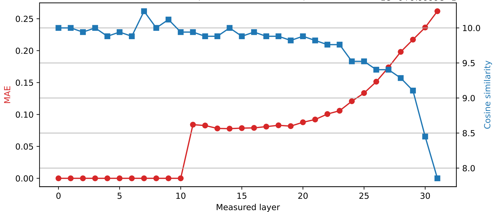
SmolLM2-360M | Quantized layer 10 | float64 → int8 1e-6+9.9999e-1
