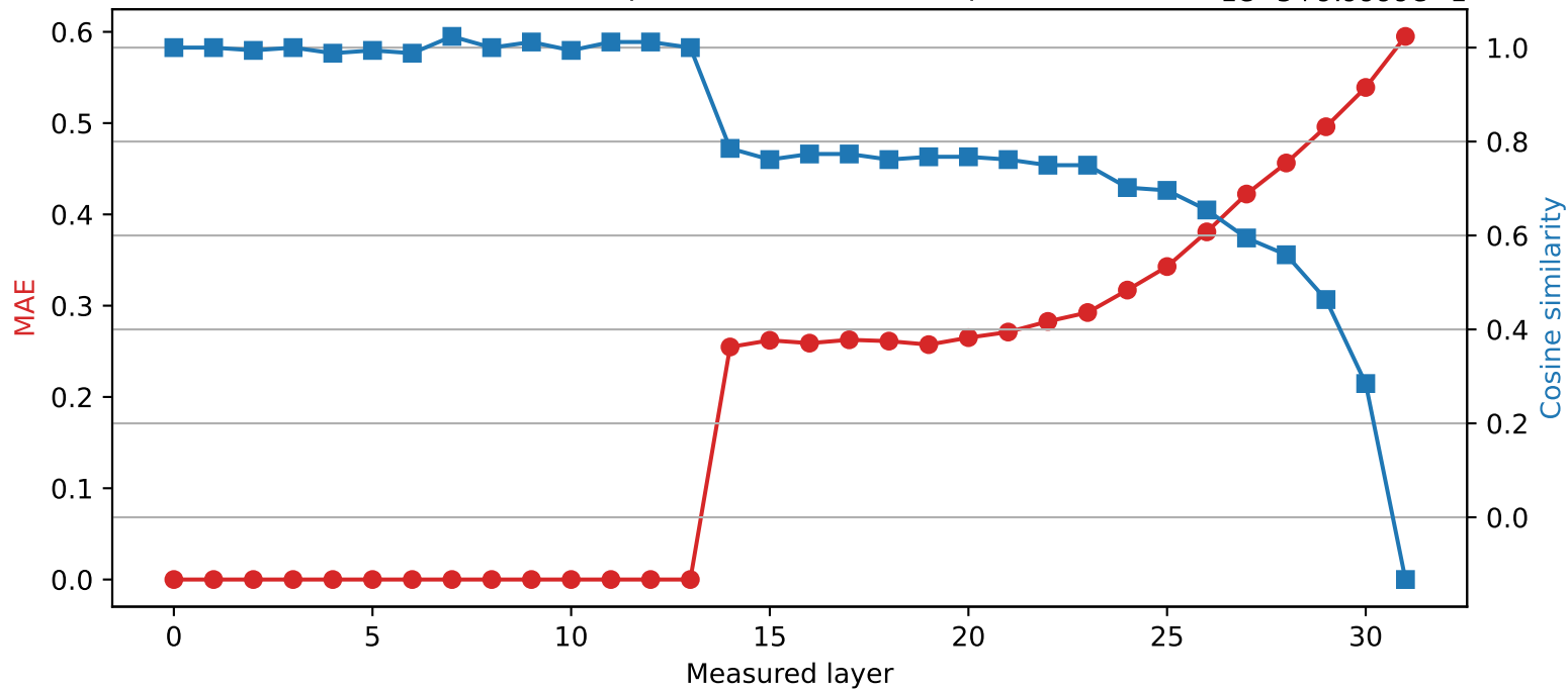
SmolLM2-360M | Quantized layer 13 | float64 \rightarrow int8 1e-5+9.9999e-1
