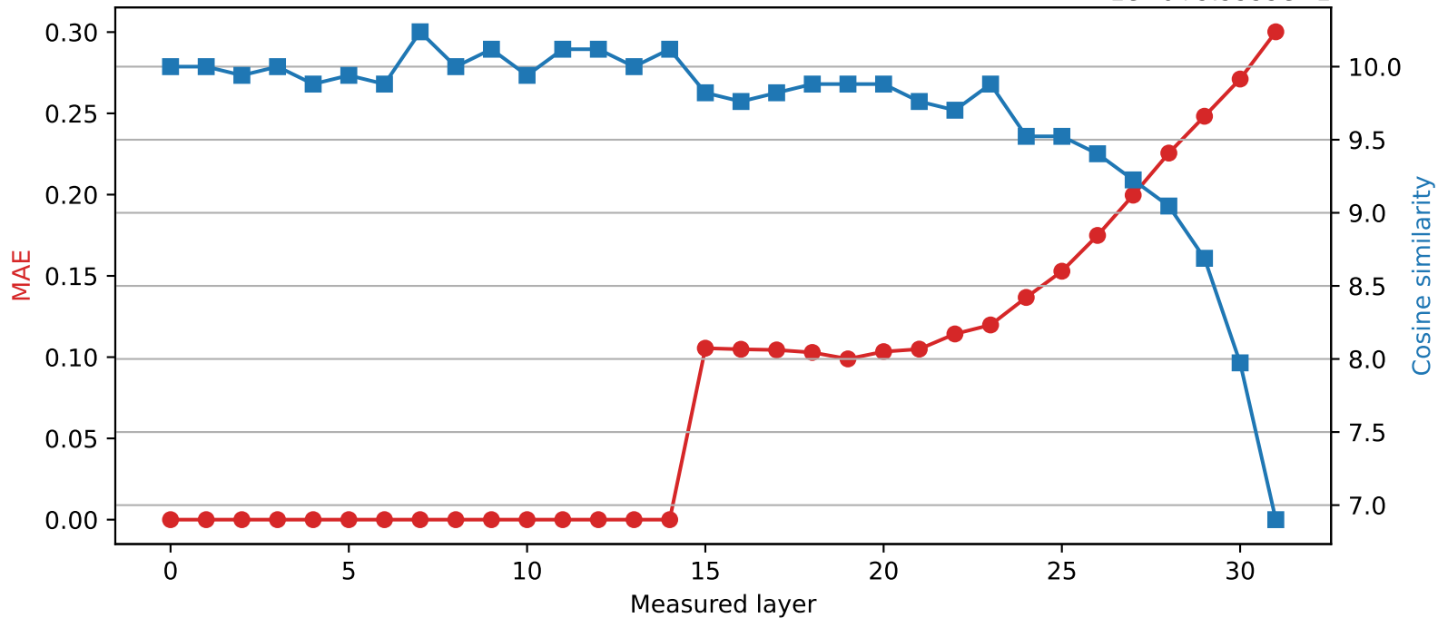
SmolLM2-360M | Quantized layer 14 | float64 → int8 1e-6+9.9999e-1
