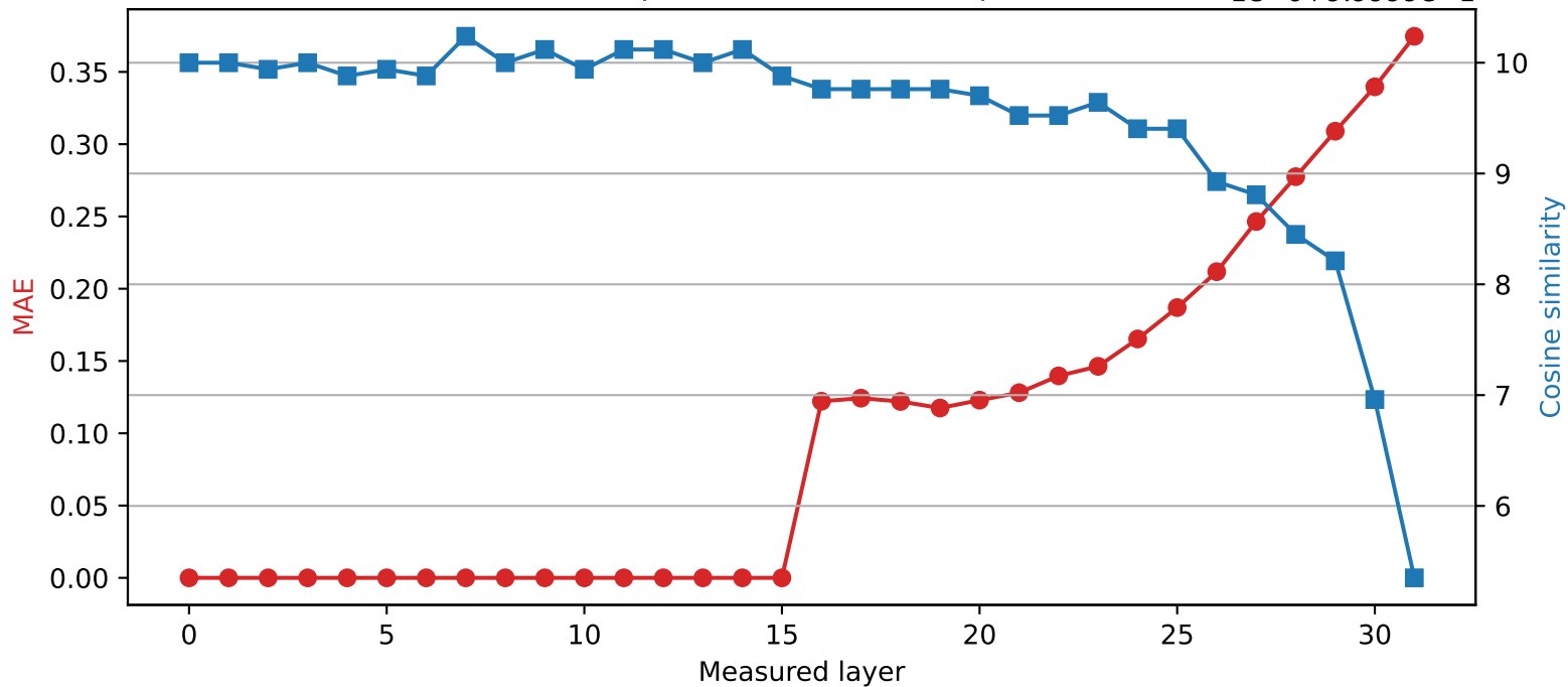
SmolLM2-360M | Quantized layer 15 | float64 \rightarrow int8 1e-6+9.9999e-1
