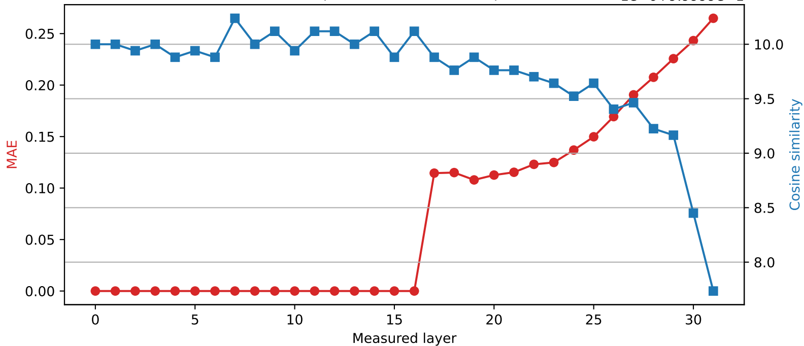
SmolLM2-360M | Quantized layer 16 | float64 \rightarrow int8 1e-6+9.9999e-1
