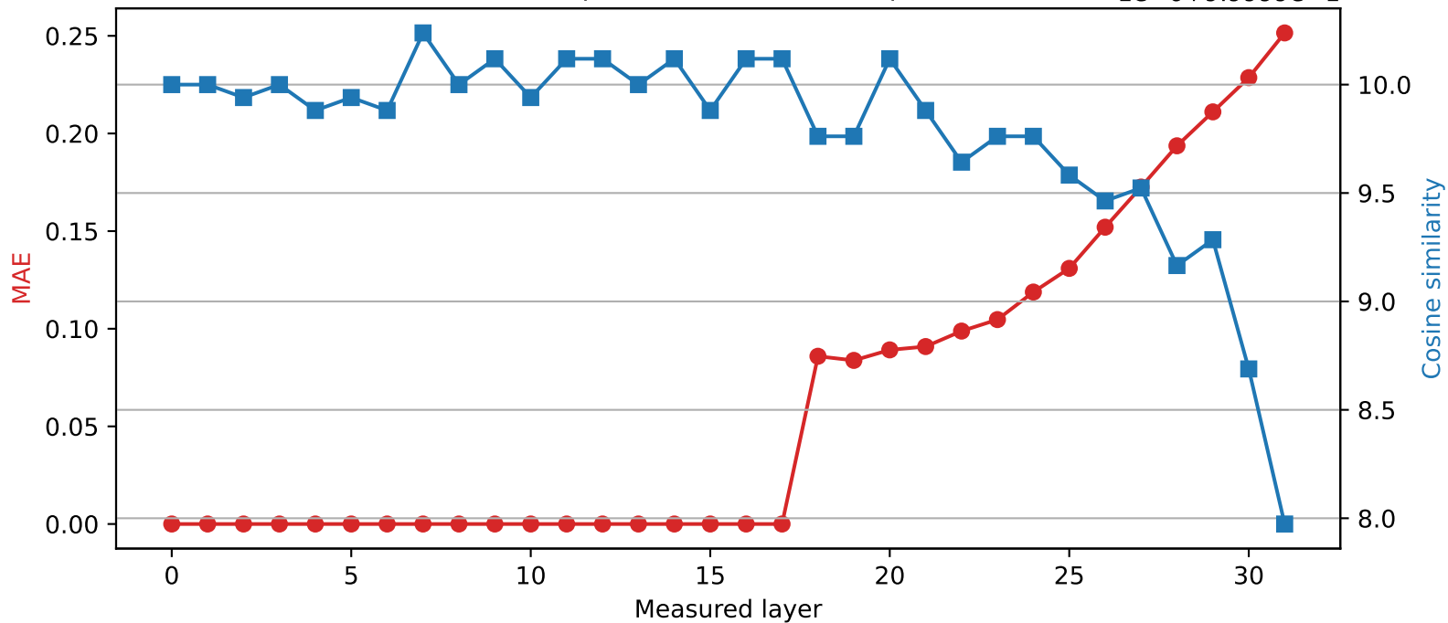
SmolLM2-360M | Quantized layer 17 | float64 \rightarrow int8 1e-6+9.9999e-1
