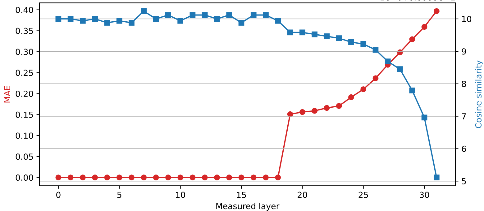
SmolLM2-360M | Quantized layer 18 | float64 → int8 1e-6+9.9999e-1
