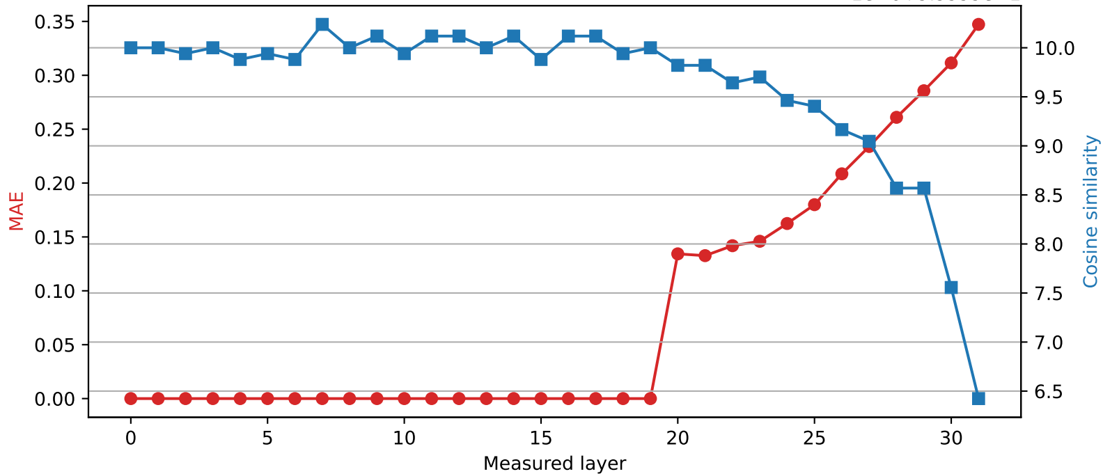
SmolLM2-360M | Quantized layer 19 | float64 → int8 1e-6 + 9.9999e-1
