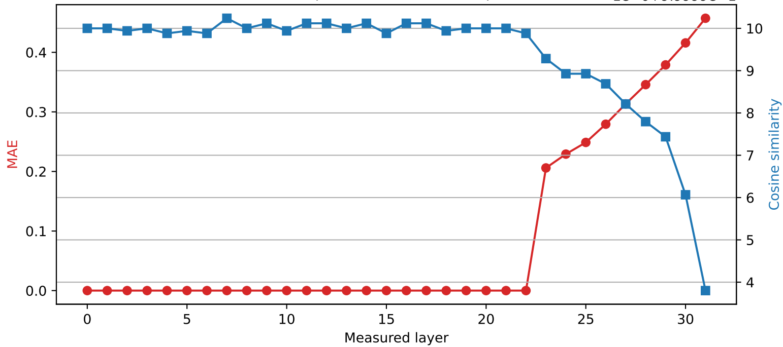
SmolLM2-360M | Quantized layer 22 | float64 → int8 1e-6 + 9.9999e-1
